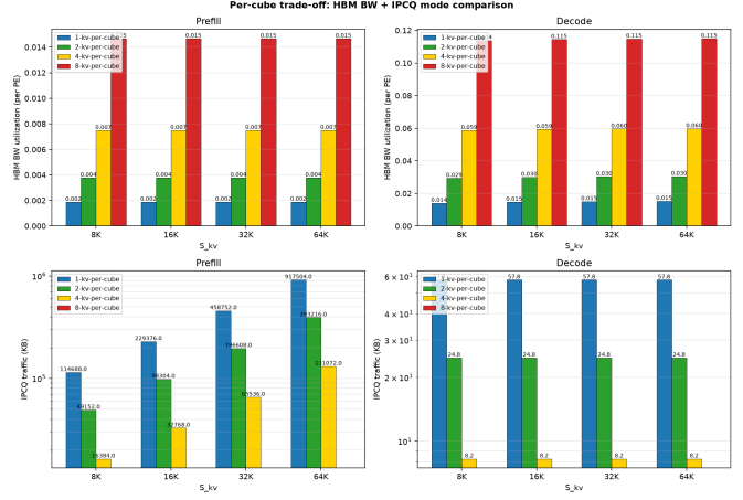
Figure 16: Per-CUBE trade-off across the four mappings (baseline kernel; HBM and IPCQ totals are variant-invariant). Top row: per-PE HBM bandwidth utilization—8-kv-per-cube concentrates roughly 8\times more bandwidth on a single CUBE than 1-kv-per-cube. Bottom row: IPCQ traffic per run on a log scale—1-kv-per-cube pays the broadcast/reduce cost across the largest group while 8-kv-per-cube (single PE per head) pays zero.
