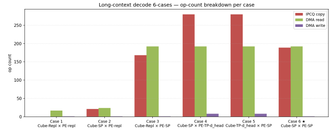
Figure 21: Measured on-device op traffic per placement. The unsharded Case 1 issues no IPCQ copies (each PE has the full cache, nothing to reduce); the single-axis Case 3 charges 168. Among the 64-way splits, the d_{\text{head-split}} Cases 4–5 charge the most—280 IPCQ copies and 8 DMA writes each, the partial-score all-reduce that head-slicing forces—while Case 6 \star needs only 189 IPCQ copies and a single DMA write, because it merges just the running softmax state (m, \ell, O) rather than partial scores. This is the on-device collective traffic that PE_IPCQ and the torus links of §4 are provisioned to absorb at link speed.
