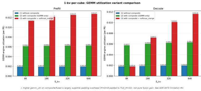
Figure 18: GEMM engine utilization on 1-kv-per-cube across the three composite tiers. The \sim 3 and \sim 6\times rise on the composite and softmax_merge tiers reflects supertile padding (the 8 \rightarrow 32 pad in M ) being accounted as GEMM time, not added useful work. With actual M = 8 , the engine is below 2% busy in all tiers—the kernel is firmly setup- and KV-bandwidth-bound at this shape.
