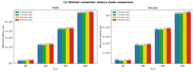
Figure 15: Wall-clock latency of the four short-context mappings, baseline kernel (no composite). Prefill and decode follow the same ordering; the two mappings are effectively tied at 8K and separate as context grows, the 8-kv-per-cube/1-kv-per-cube ratio widening from 0.98\times at 8K to 1.06\times at 64K (1-kv-per-cube faster at the large end). The composite and softmax_merge tiers track the baseline within a few percent at this shape (see Figure 17).
