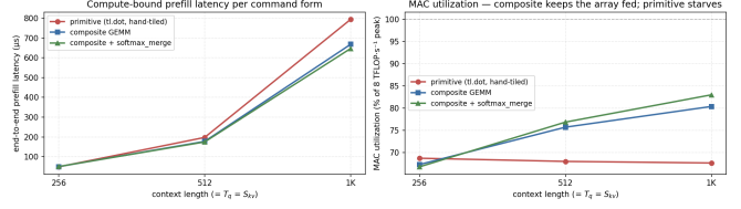
Figure 23: Compute-bound prefill, three command forms, swept over context length ( M=8 T_q tile-filling). Left: end-to-end latency. Right: MAC utilization (achieved \div the 8 \text{ TFLOPs}^{-1} per-PE peak). The hand-tiled primitive sits flat at \sim 68\% —its serial load \rightarrow dot path leaves the MAC array idle between tiles regardless of context. The composite forms climb with context (67 \rightarrow 80% plain, 67 \rightarrow 83% with the recipe) because a deeper P-V reduction gives more HW tiles to pipeline, and they convert that into wall-clock: at 1024 the recipe form is 646.9 vs. 794.1 \mu\text{s} (19% faster). The margin grows with context—the compute-bound mirror of the GEMM result of §3.
